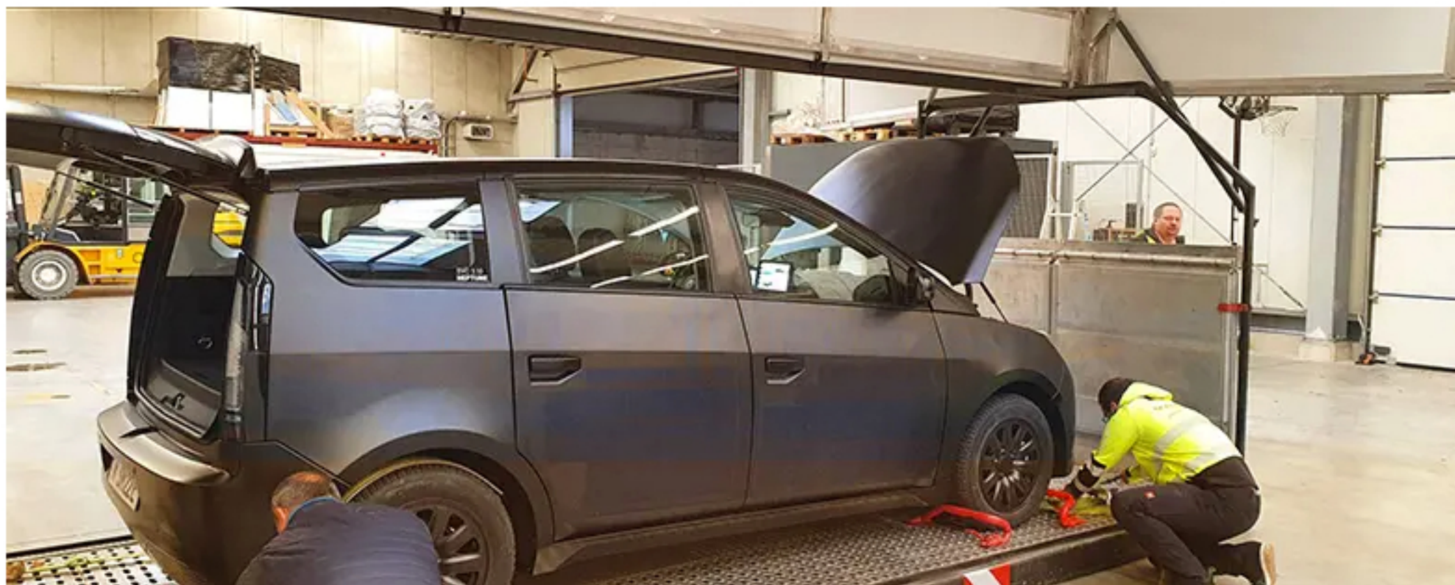
The solar-powered SION is fitted into the patented and unique ATBneo automotive transportation box before its US journey.
